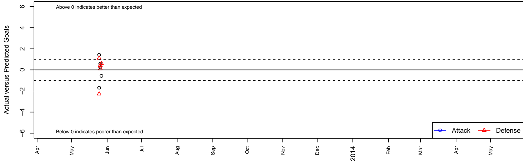
Mad River United Rangers B02 Dots are actual minus expected GF (blue circles) and GA (red triangles). Blue line is smoothed change in attack strength. Red is smoothed change in defense strength.
